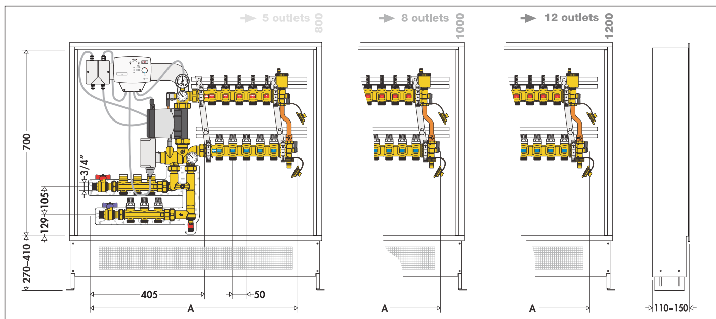
Dimensions of modulating temperature regulating unit with digital regulator and medium distribution kit for primary circuit 171 series
