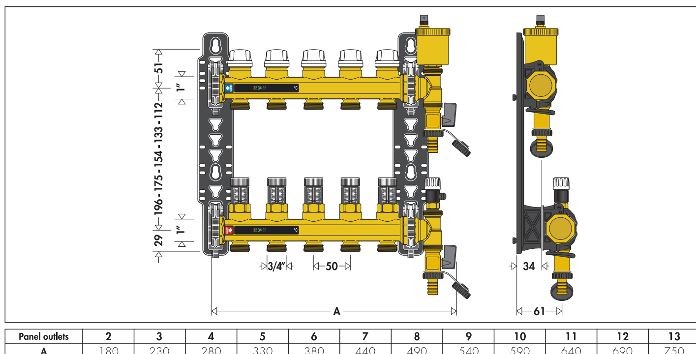
Dimensions of pre-assembles distribution manifolds 662 series with micrometric valves
