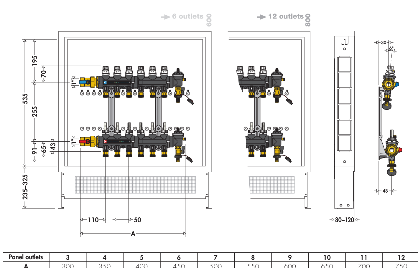
Dimensions of manifolds 670 series
