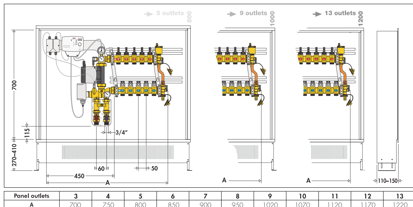
Dimensions of modulating temperature regulating unit with digital regulator 171 series
