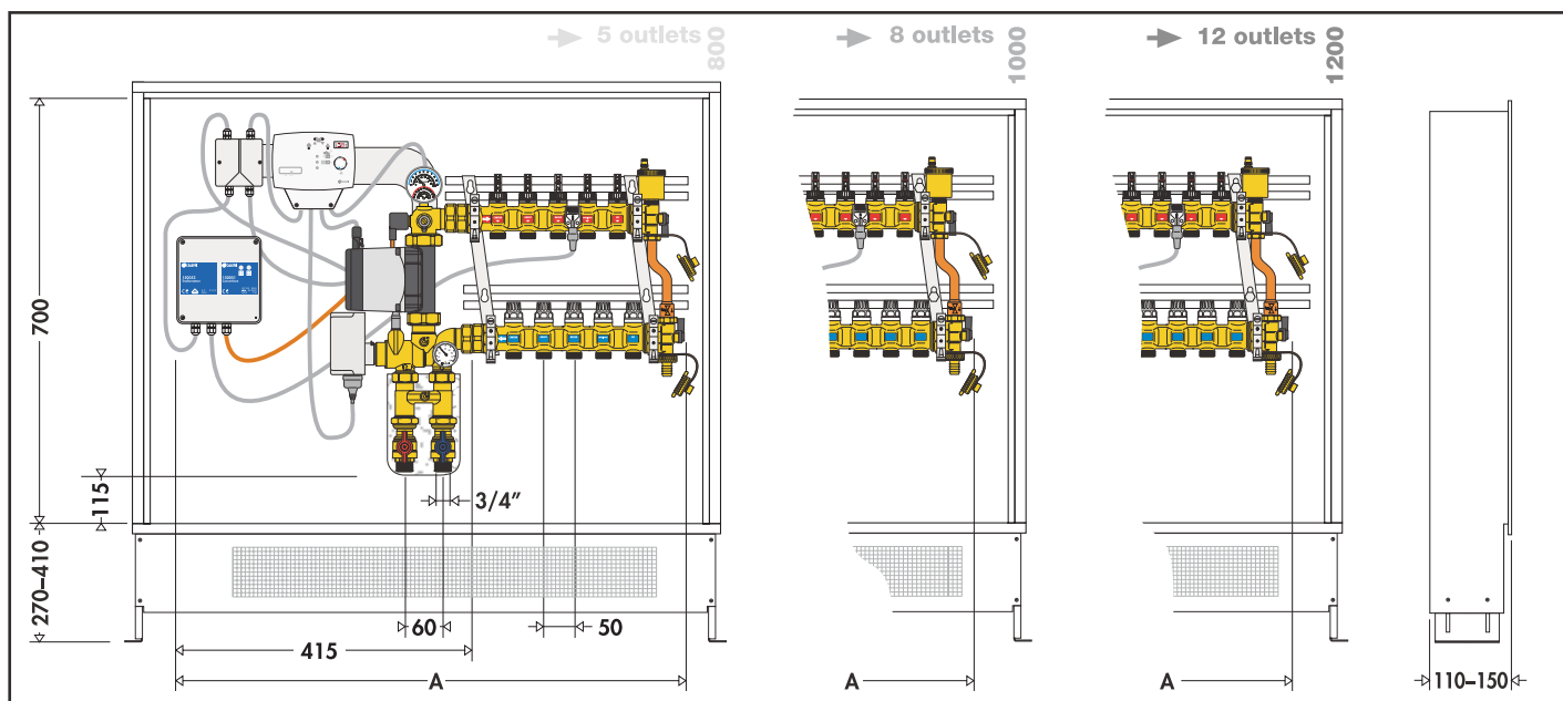
Dimensions of modulating temperature regulating unit with digital regulator for heating and cooling 171 series
